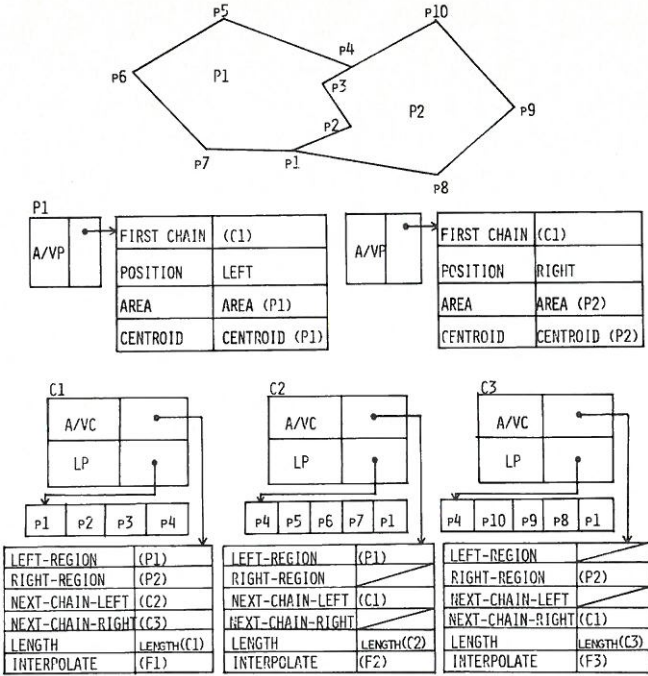
Figure 2 illustrates a spatial data structure for a simple map that encompasses the structures used in the Canada Geographic Information System, the DIME System, the POLYVRT system, and LJUDA system.
