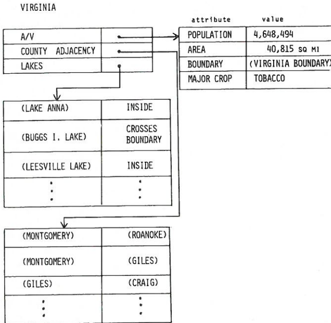
Figure 1 illustrates a spatial data structure representing the state of Virginia.
