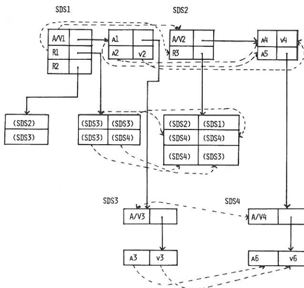
Figure 8 illustrates a homomorphism from spatial data structure SDS1 to spatial data structure SDS2.
