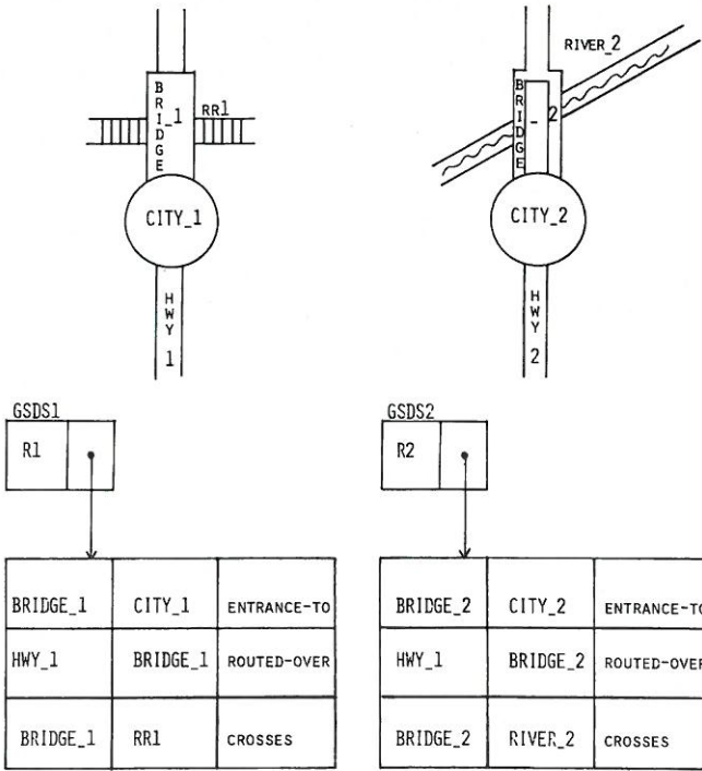
Figure 9 illustrates two geographic spatial data structures that are similar at least at the top level.
