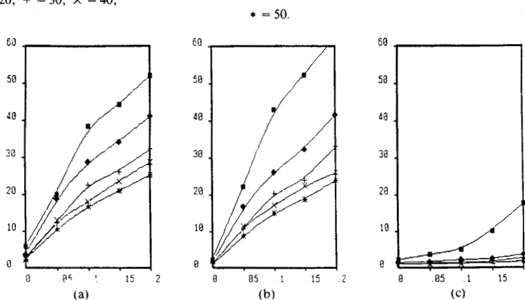
Fig. 13. Illustrates performance characteristics of angle error versus fraction of outliers for initial approximation method, linearized least-squares adjustment, and robust M -estimate. Refer to Fig. 12 for legend.
