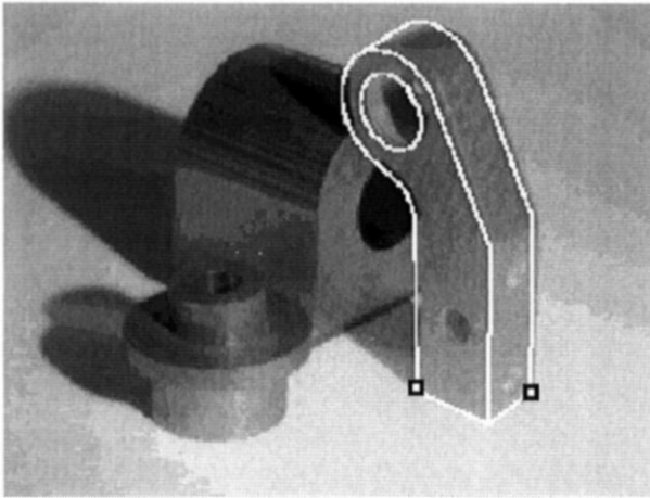
Fig. 12. The pose computed using two points (as indicated by the black squares) and one circle (the upper circle) with the integrated technique.
