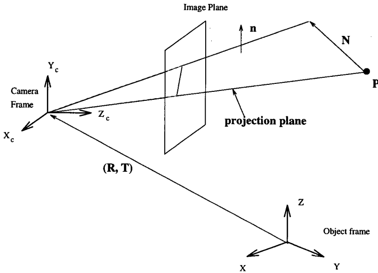
Fig. 2. Projection plane formed by a 2D image line l and the corresponding 3D line L .
