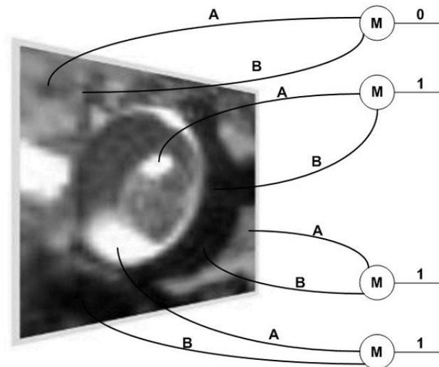
Fig. 7. Shows Minchinton Cells. As seen from the example preprocessing elements, M cells sample two indexes from the data, and produce either binary 1 or 0 based on the comparison of point A and B: adapted from [48]
